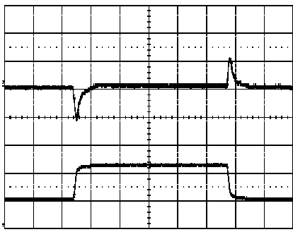
Output voltage response to load current step- change (25-50-25 A) at: T_{ref} = +25^{\circ}\text{C} , V_i = 12.0\text{ V} . Top trace: output voltage (100 mV/div.). Bottom trace: load current (20 A/div.). Time scale: 0.2 ms/div.
