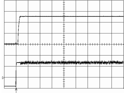
Start-up enabled by connecting V_i at: T_{ref} = +25^\circ\text{C} , I_o = 50\text{ A} resistive load, V_i = 12.0\text{ V} . Top trace: output voltage (2.0 V/div.). Bottom trace: input voltage (5 V/div.). Time scale: 20 ms/div.
