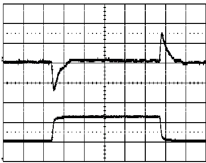
Output voltage response to load current step- change (25-50-25 A) at: T_{ref} = +25^\circ\text{C} , V_i = 12.0\text{ V} . Top trace: output voltage (100 mV/div.). Bottom trace: load current (20 A/div.). Time scale: 0.2 ms/div.
