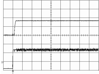
Start-up enabled by connecting V_i at: T_{ref} = +25^{\circ}\text{C} , I_o = 50\text{ A} resistive load, V_i = 12.0\text{ V} . Top trace: output voltage (2.0 V/div.). Bottom trace: input voltage (5 V/div.). Time scale: 20 ms/div.
