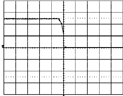
Shut-down enabled by disconnecting V_i at: T_{ref} = +25^\circ\text{C} , I_o = 50\text{ A} resistive load, V_i = 12.0\text{ V} . Top trace: output voltage (2.0 V/div.). Time scale: 1.0 ms/div.
