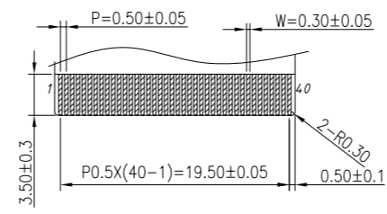
A Detail
