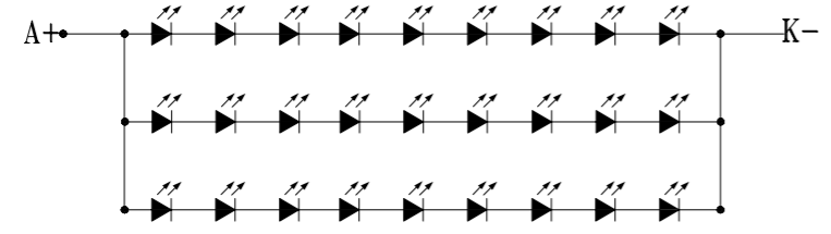
WHITE LED 60mA/27.0V(TYP) LED CIRCUIT DIAGRAM:
