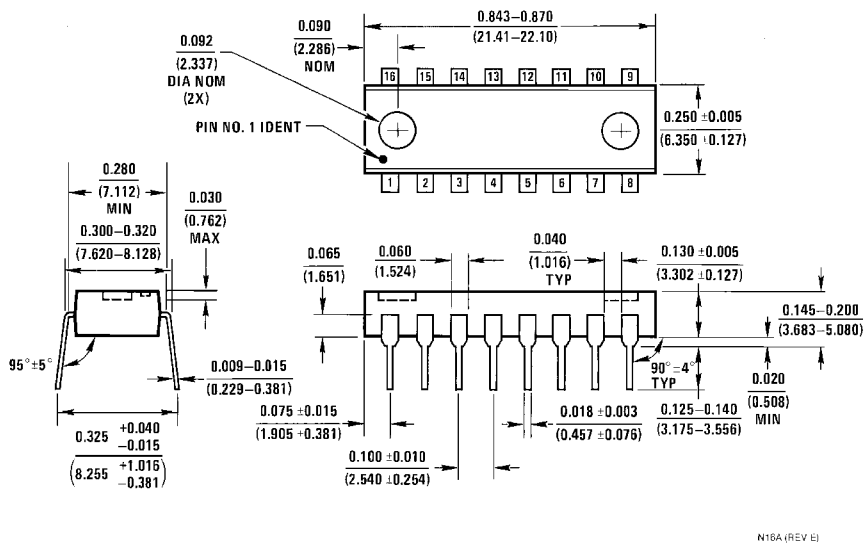
16-Pin Molded Dual-In-Line Package Order Number LMC6684AIN or LMC6684BIN NS Package Number N16A
