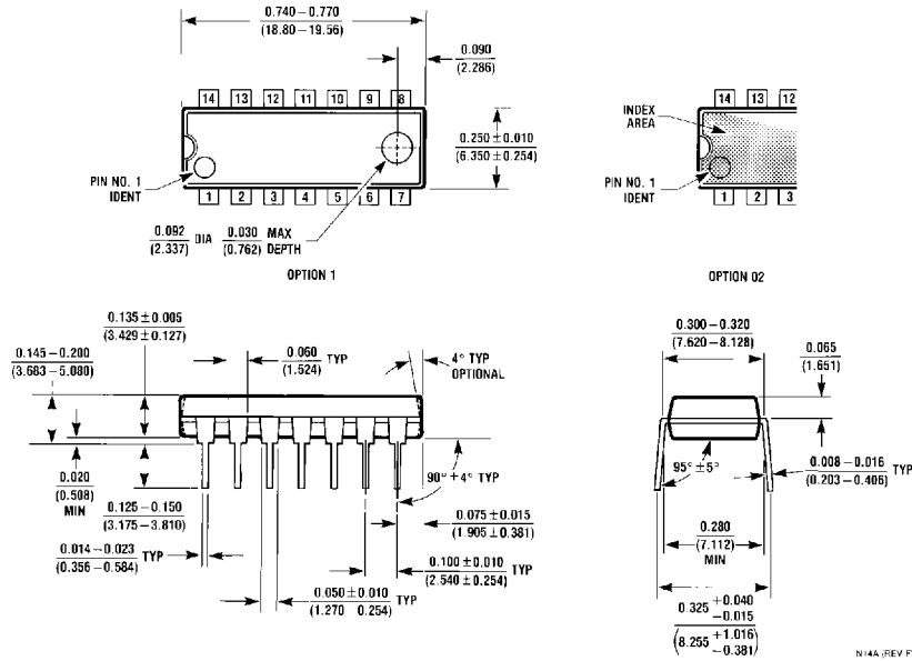
14-Pin Molded Dual-In-Line Package Order Number LMC6682AIN or LMC6682BIN NS Package Number N14A
