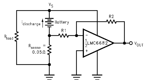
FIGURE 27. Circuit Used to Sense Discharging
