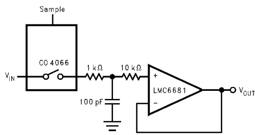
FIGURE 25. Sample-and-Hold Application
