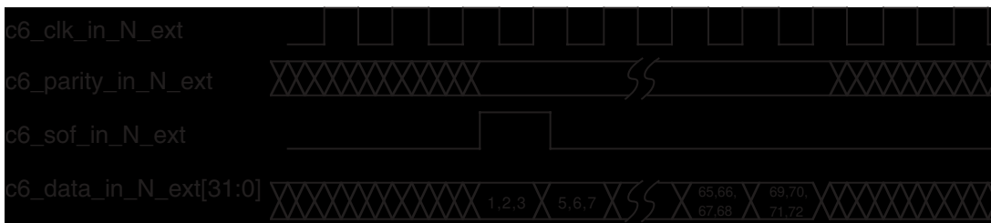
Figure 2. CSIX Inbound Frame Transfer
