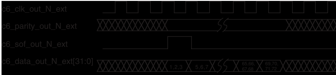
Figure 4. CSIX Outbound Frame Transfer
