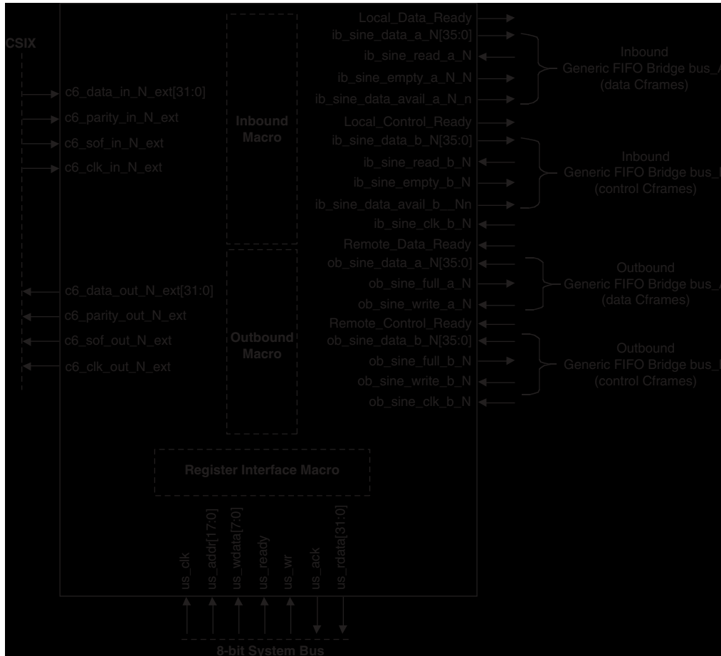
Figure 1. Simplified Block Diagram - CSIX Level 1 Core
