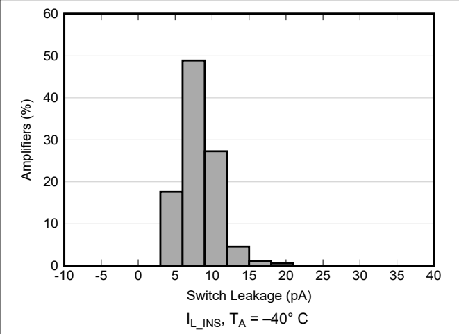
Figure 6-37. Switch Input Leakage Current Histogram
