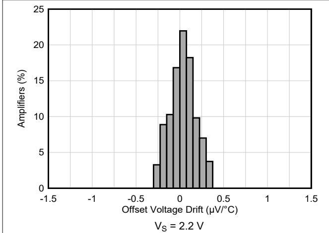
Figure 6-4. Offset Voltage Drift Distribution
