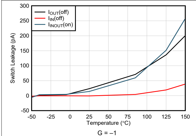
Figure 6-36. Switch Leakage Current vs Temperature
