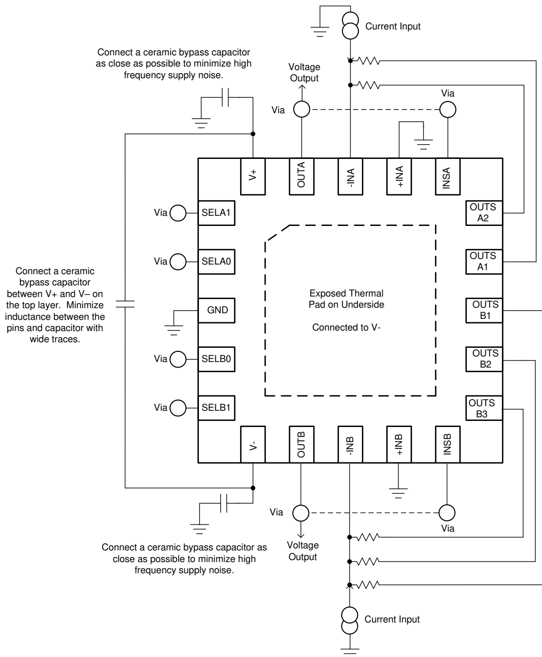
Figure 11-1. Layout Example
