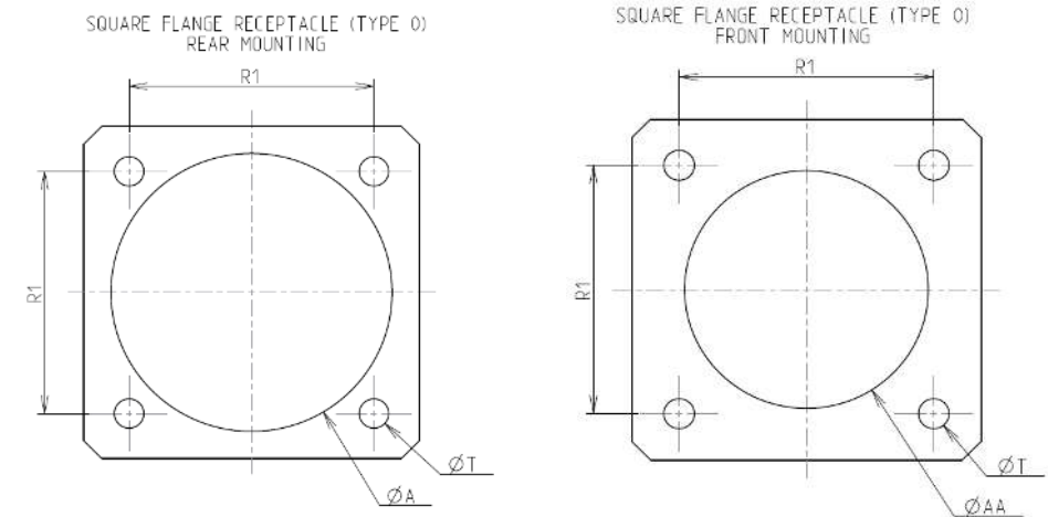
Panel Cutout
