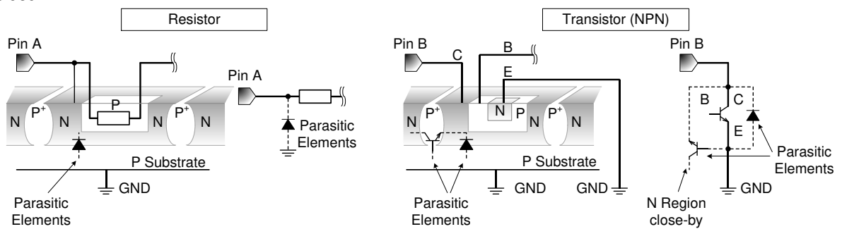
Figure 33. Example of IC structure
