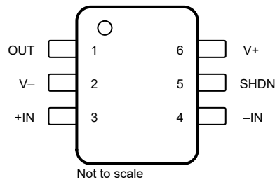
Figure 5-3. TLV9161S DBV Package 6-Pin SOT-23 (Top View)
