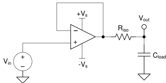
Figure 7-7. Extending Capacitive Load Drive With the TLV9161
