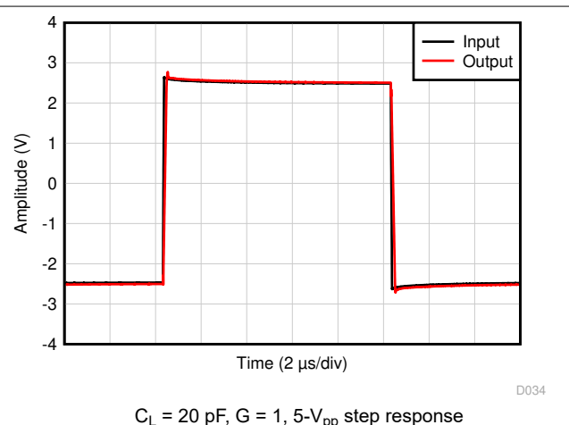
Figure 6-36. Large-Signal Step Response
