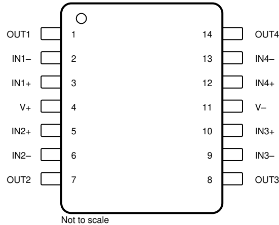
Figure 5-7. TLV9164 D and PW Package 14-Pin SOIC and TSSOP (Top View)
