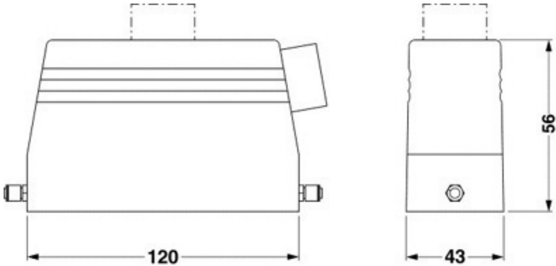
Dimensioned drawing
