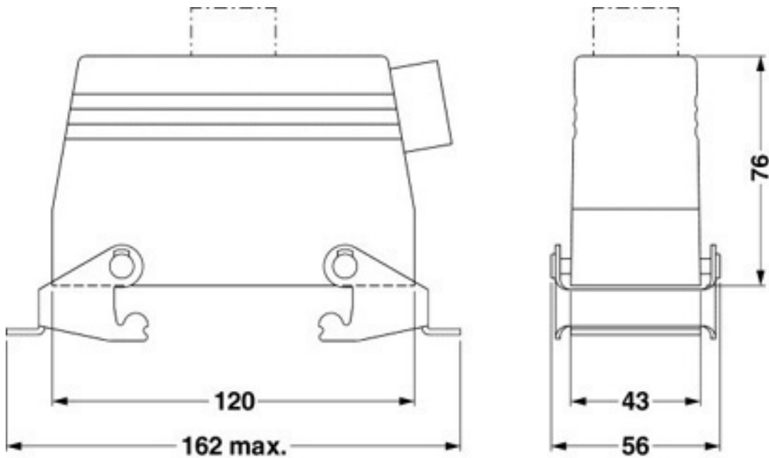
Dimensioned drawing
