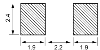
Figure 2) Suggested land
