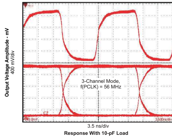
Figure 6-13. XGA 3-Channel Output Waveform
