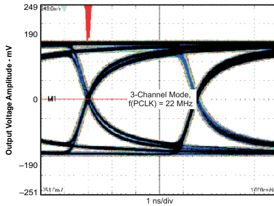
Figure 9-8. VGA3-Channel Output Waveform
