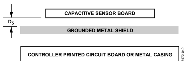
Figure 43. Capacitive Sensor Board Mechanicals Side View
