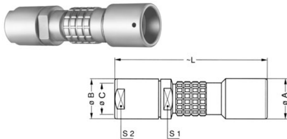
PHG Free socket, nut fixing, with key (G) or keys (code A to F and L) and oversize collet – watertight
