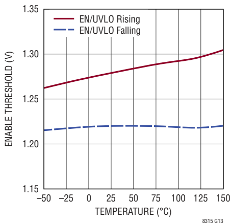
EN/UVLO Threshold
