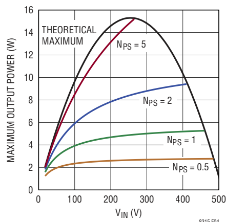
Figure 4. Maximum Power, V_{OUT} = 48V
