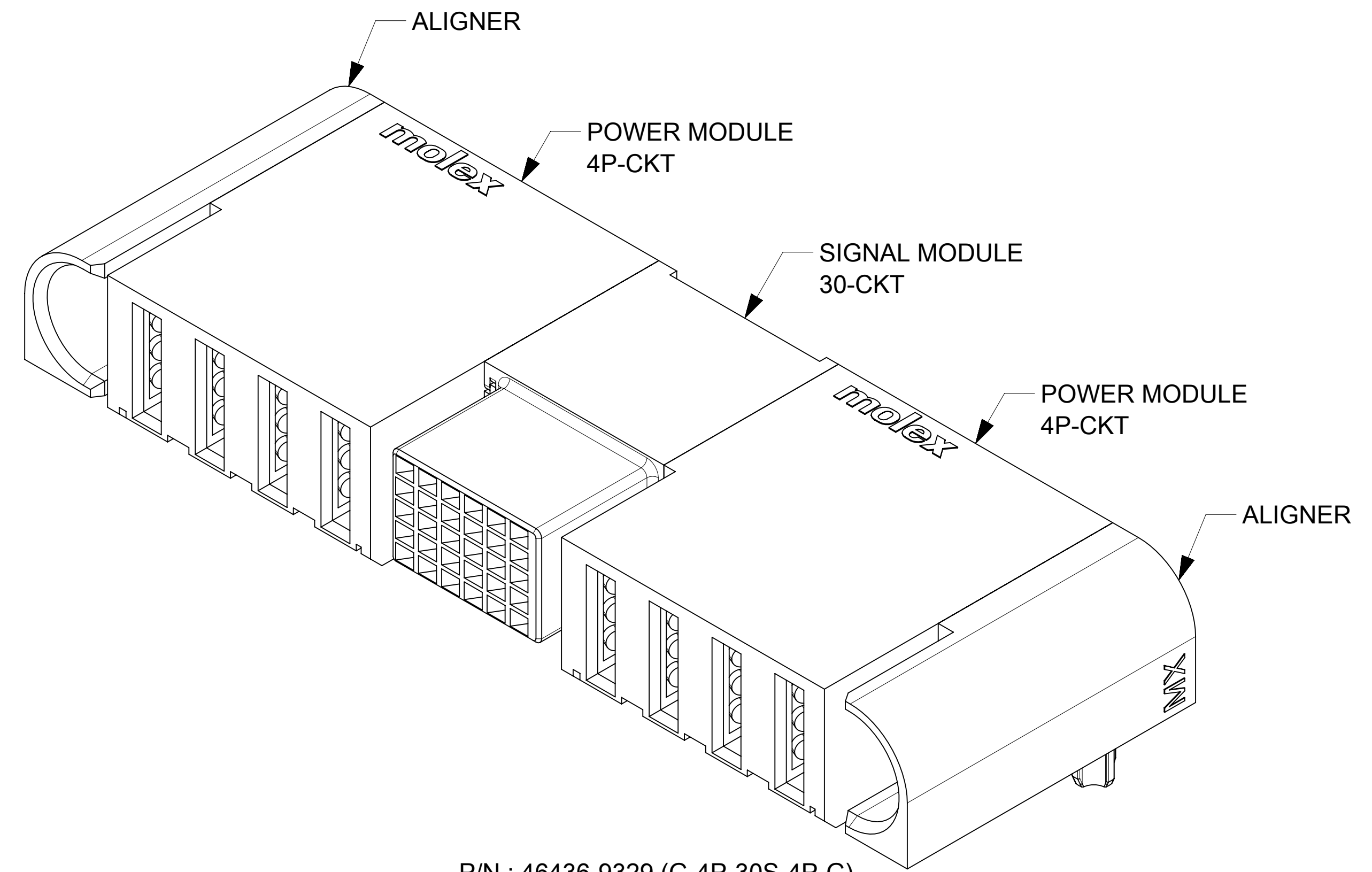
P/N : 46436-9329 (G-4P-30S-4P-G)
