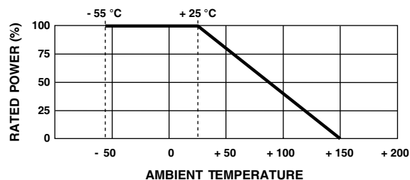
FIGURE 5 – POWER DERATING CURVE
