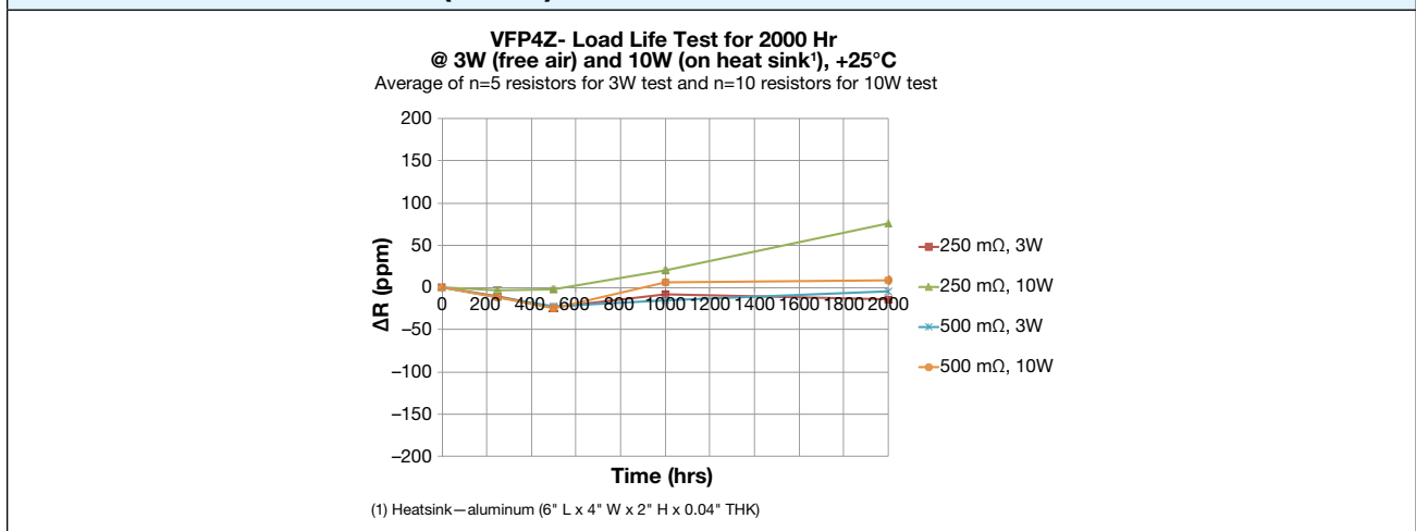
FIGURE 8 – LOAD LIFE TEST (VFP4Z)
