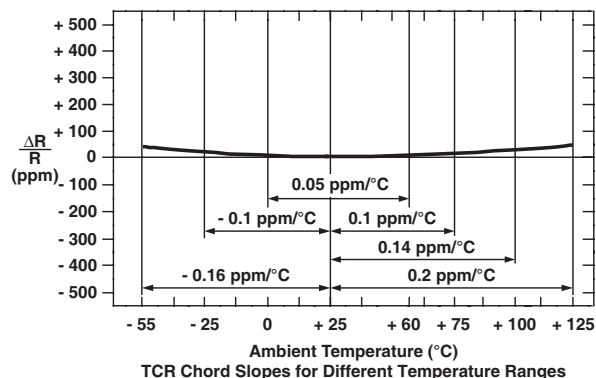
FIGURE 4 – TYPICAL RESISTANCE/TEMPERATURE CURVE (Z-FOIL)
