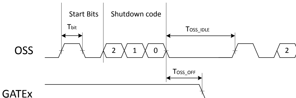
Figure 2.7. OSS Pin in Multi-Bit Mode
