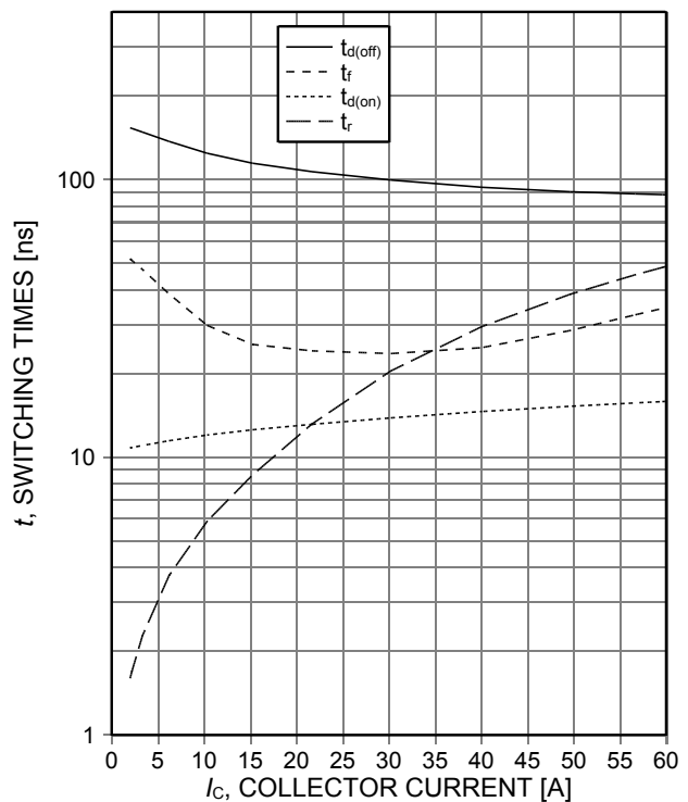
Figure 8. Typical switching times as a function of collector current (inductive load, T_{vj}=150^\circ\text{C} , V_{CE}=400\text{V} , V_{GE}=15/0\text{V} , r_G=32\Omega , Dynamic test circuit in Figure E)
