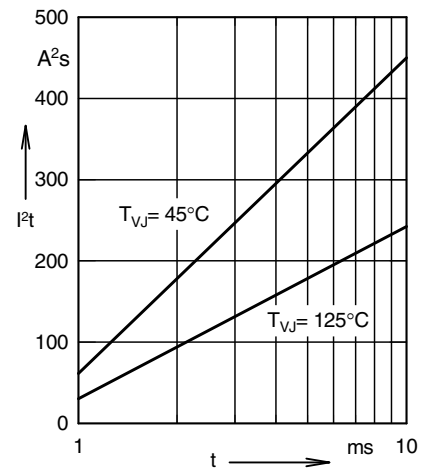
Fig. 2 I²t for fusing (Rectifier Diodes)
