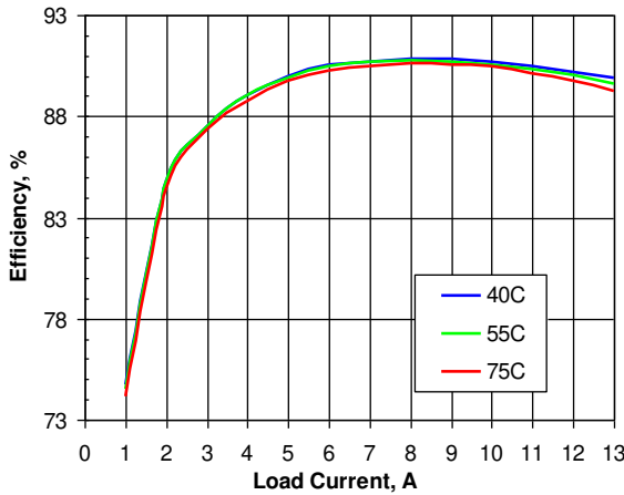
Figure 3 Efficiency vs. load current and ambient temperature for SSQE48T13050 converter mounted vertically with V_{in} = 48 V and air flowing from pin 1 to pin 3 at a rate of 200 LFM (1.0 m/s).
