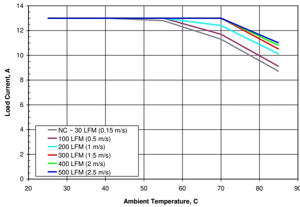
Figure 1. Available load current vs. ambient air temperature and airflow rates for SSQE48T13050 converter mounted vertically with air flowing from pin 1 to pin 3, V_{in} = 48 V . Note: NC – Natural convection
