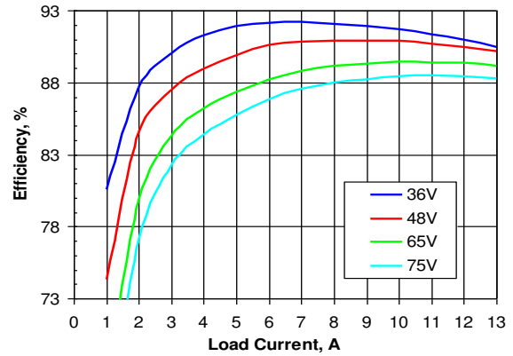
Figure 2. Efficiency vs. load current and input voltage for SSQE48T13050 converter mounted vertically with air flowing from pin 1 to pin 3 at a rate of 300 LFM (1.5 m/s) and T_a = 25^\circ C .
