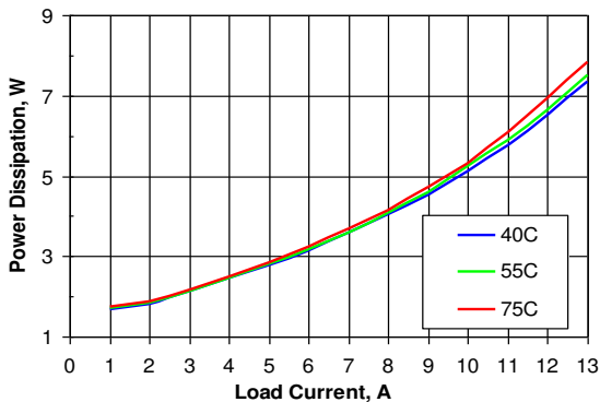
Figure 5. Power dissipation vs. load current and ambient temperature for SSQE48T13050 converter mounted vertically with V_{in} = 48 V and air flowing from pin 1 to pin 3 at a rate of 200 LFM (1.0 m/s).
