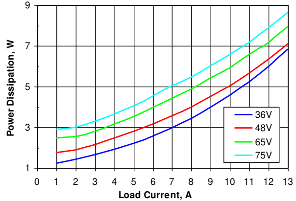
Figure 4. Power dissipation vs. load current and input voltage for SSQE48T13050 converter mounted vertically with air flowing from pin 1 to pin 3 at a rate of 300 LFM (1.5 m/s) and T_a = 25^\circ C
