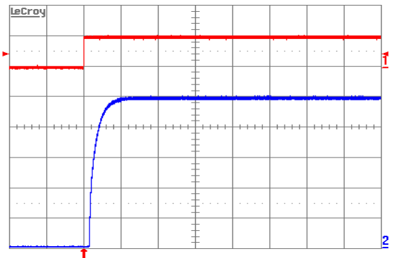
Figure 6. Turn-on transient at full rated load current (resistive) with no output capacitor at V_{in} = 48 V , triggered via ON/OFF pin. Top trace: ON/OFF signal (5 V/div.). Bottom trace: Output voltage (1.0 V/div.). Time scale: 5 ms/div.
