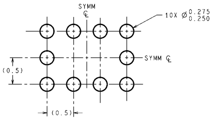
16-Lead Thin Leadless Leadframe Package NS Package Number SQA16A
