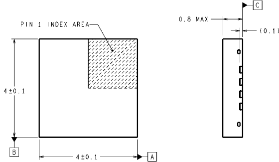
16-Lead Thin Leadless Leadframe Package NS Package Number SQA16A
