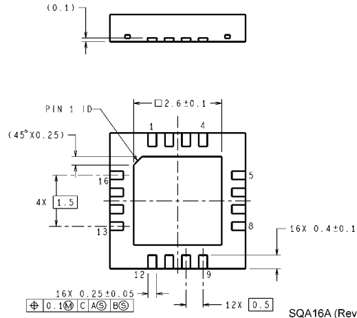
16-Lead Thin Leadless Leadframe Package NS Package Number SQA16A
