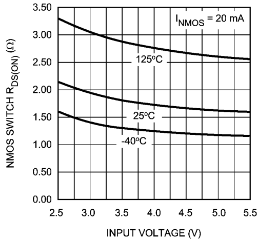
NMOS R_{DS(ON)} (Figure 2: N2) vs V_{IN}
