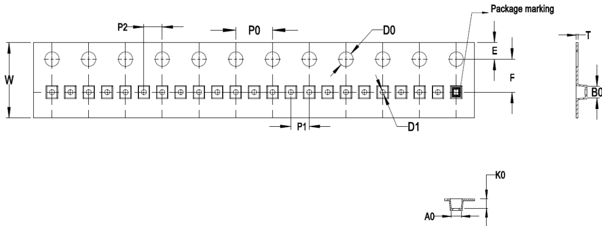
Figure 12: Carrier Tape Drawing
