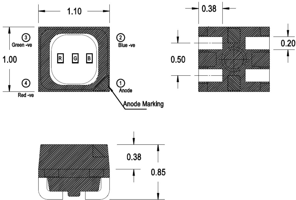
Figure 1: Package Drawing
