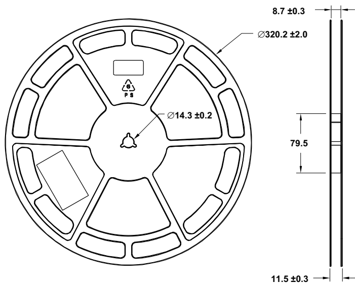
Figure 13: Reel Drawing
