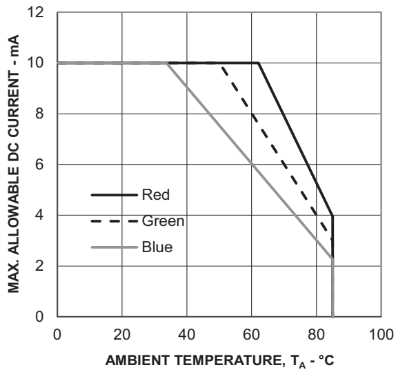
Figure 8: Maximum Forward Current vs. Temperature for Red, Green, and Blue (Three Chips On)
