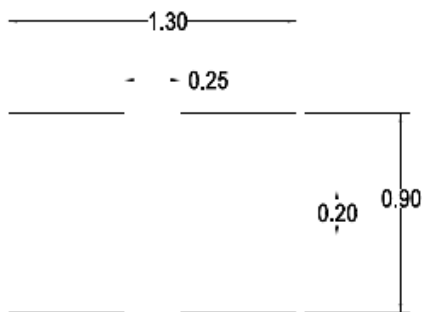
Figure 11: Recommended Soldering Pad Pattern
