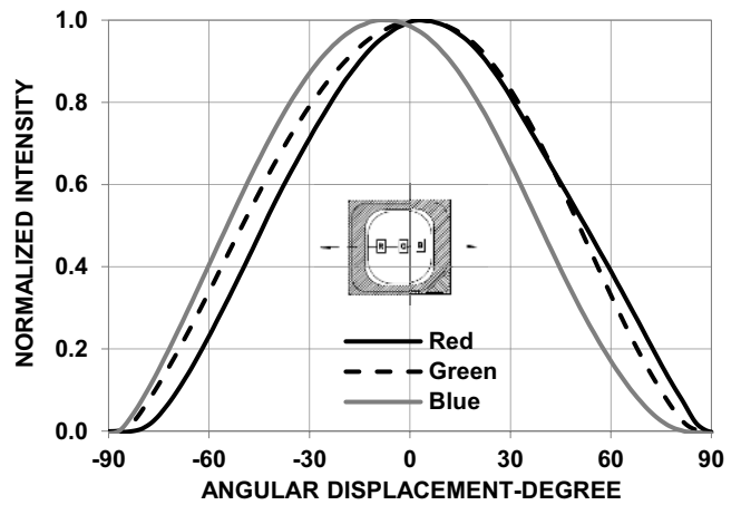
Figure 10: Radiation Pattern for y-axis
