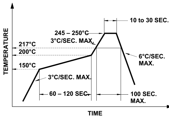
Figure 14: Recommended Lead-Free Reflow Soldering Profile
