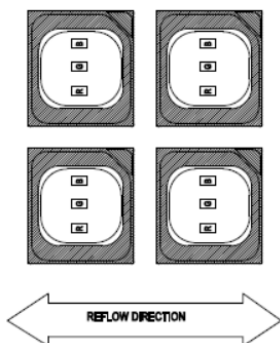
Figure 15: Recommended Board Reflow Direction
