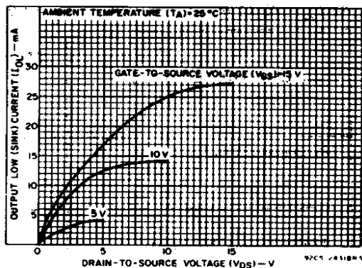
Figure 5. Typical Output Low (Sink) Current Characteristics
