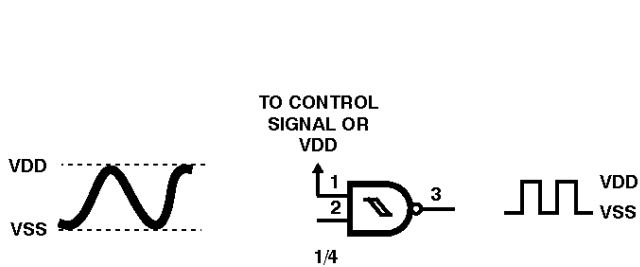
FREQUENCY RANGE OF WAVE SHAPE IS FROM DC TO 1MHz
