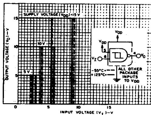
Figure 4. Typical Voltage Transfer Characteristics as a Function of Temperature
