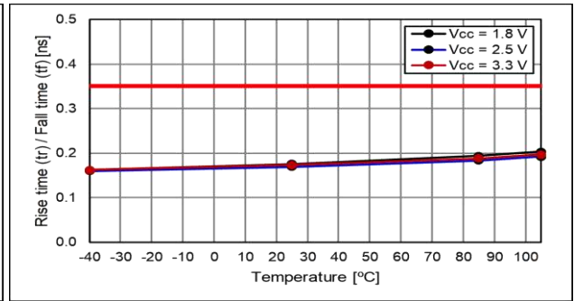
Fall Time
