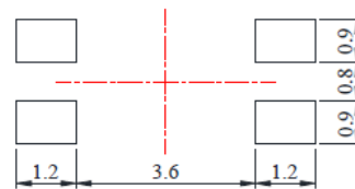
Figure 1. IN-P32TRRRGB Solder Pattern
