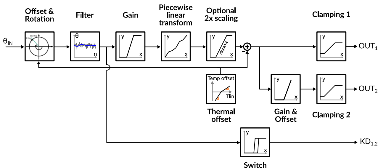
fig. 18 – MLX90374 Digital Processing Flow
