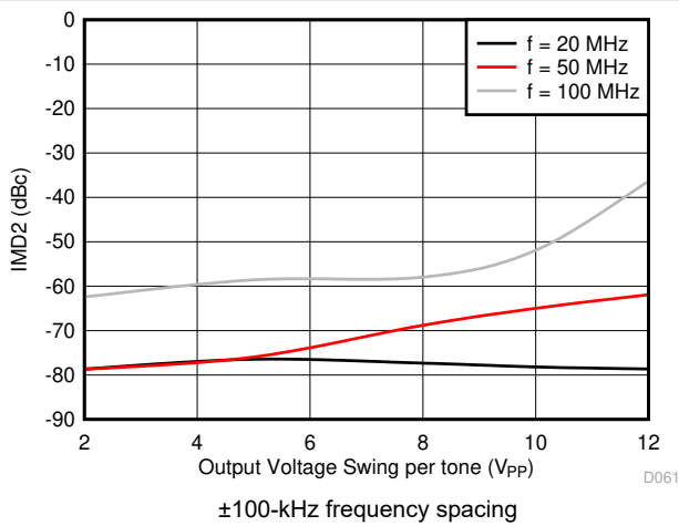
Figure 8-19. IMD2 vs Output Voltage Swing
