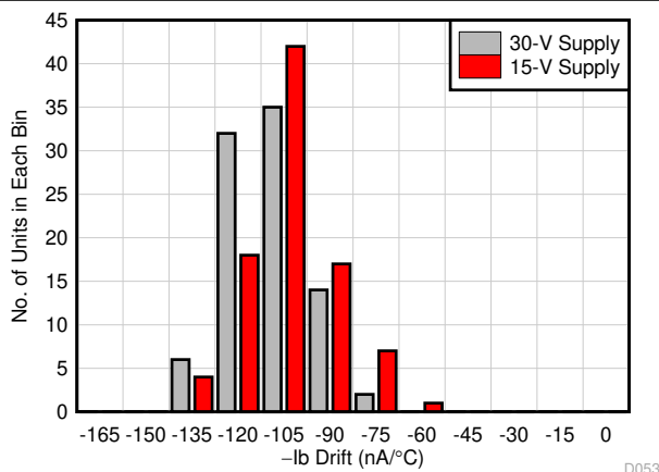
Figure 8-37. Noninverting I_B Over Temperature
