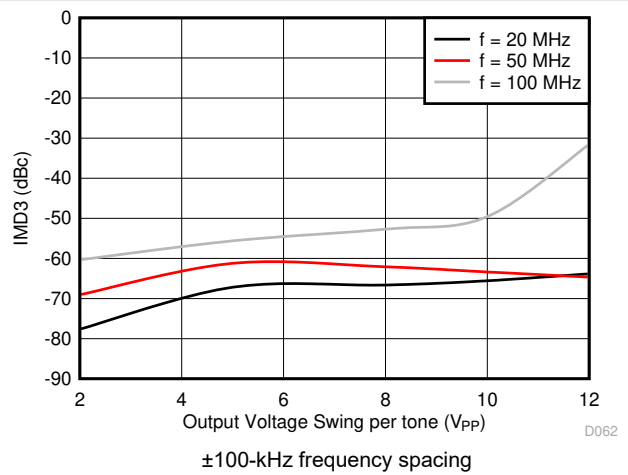
Figure 8-20. IMD3 vs Output Voltage Swing
