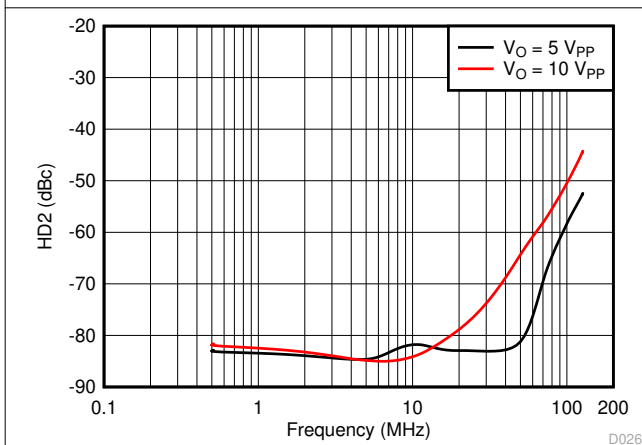
Figure 8-46. HD2 vs Frequency Across Output Swing
