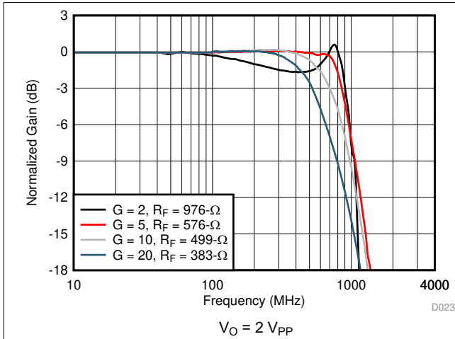
Figure 8-42. Noninverting Small-Signal Frequency Response
