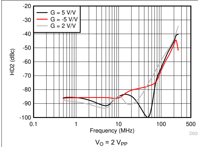
Figure 8-44. HD2 vs Frequency
