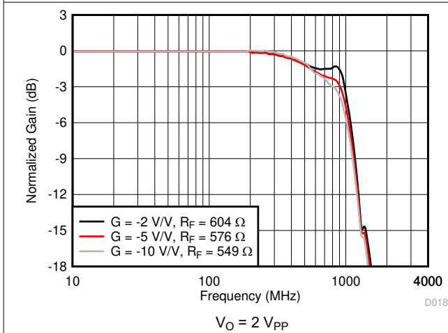
Figure 8-3. Inverting Small-Signal Frequency Response
