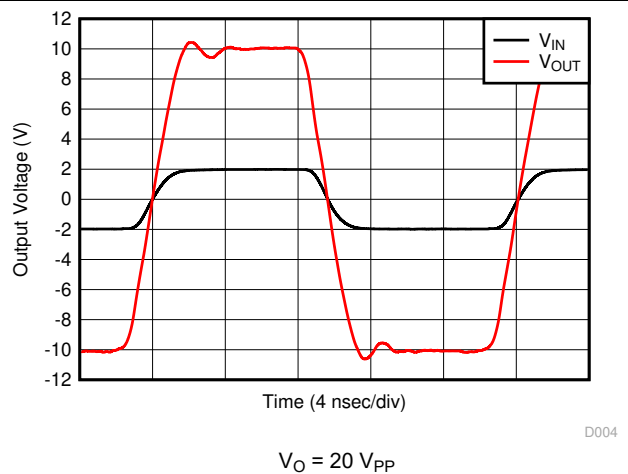
Figure 8-24. G = 5\text{ V/V} Pulse Response
