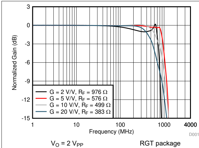
Figure 8-1. Noninverting Small-Signal Frequency Response
