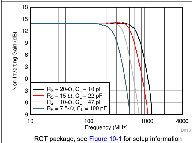
Figure 8-5. Frequency Response vs C_{LOAD}
