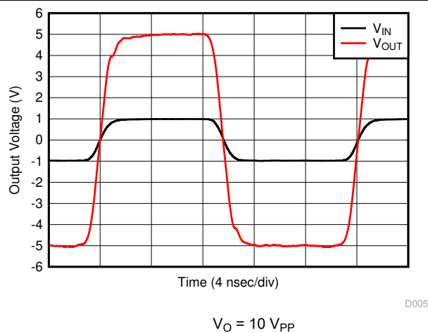
Figure 8-23. G = 5\text{ V/V} Pulse Response
