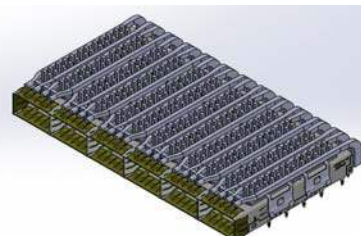
1x6 Cage with square pin heat sinks and quad barrel light pipes
