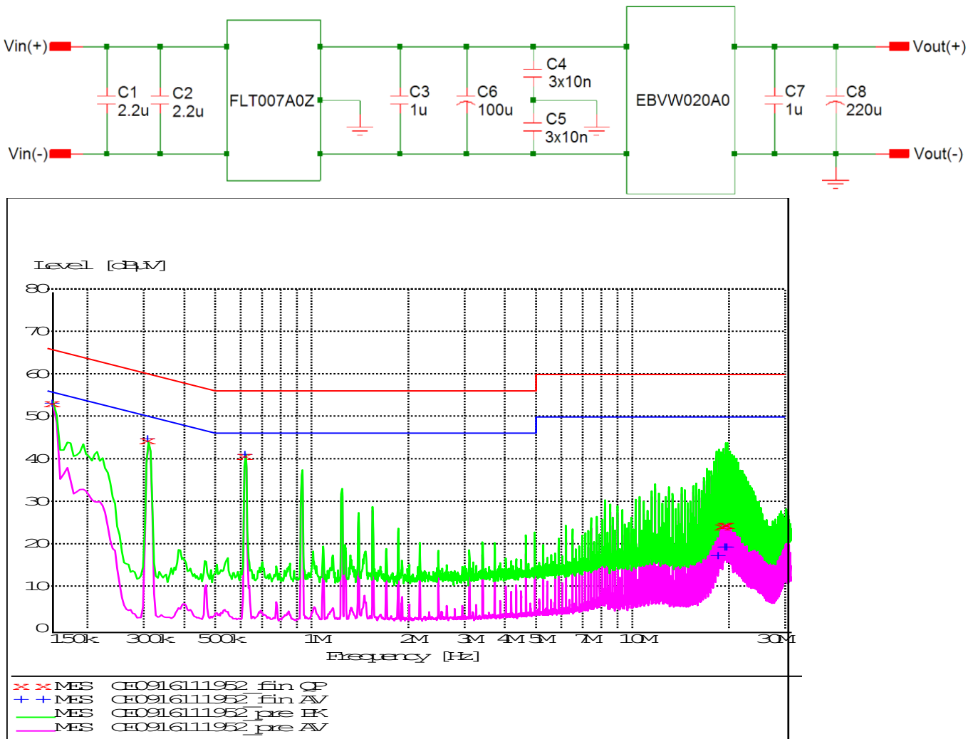
Figure 24. EMC Considerations.
