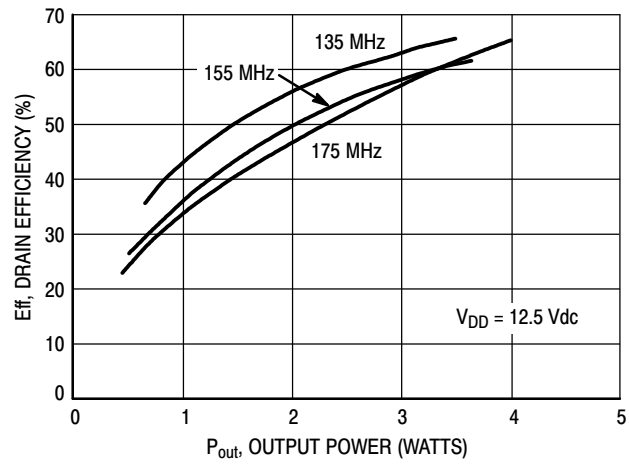
Figure 23. Drain Efficiency versus Output Power
