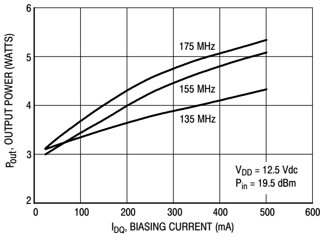
Figure 24. Output Power versus Biasing Current
