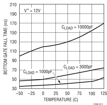
Bottom Gate Fall Time vs Temperature
