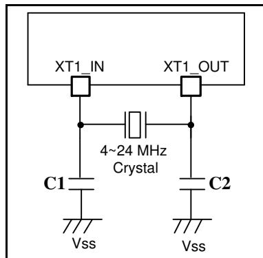
Figure 7.3-3 Typical HXT Crystal Application Circuit
