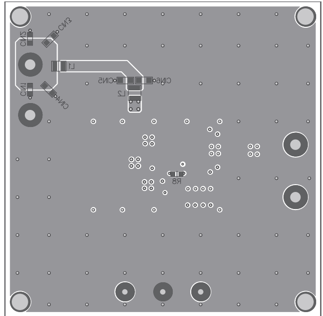
Figure 6: Bottom Layer and Bottom Silk
