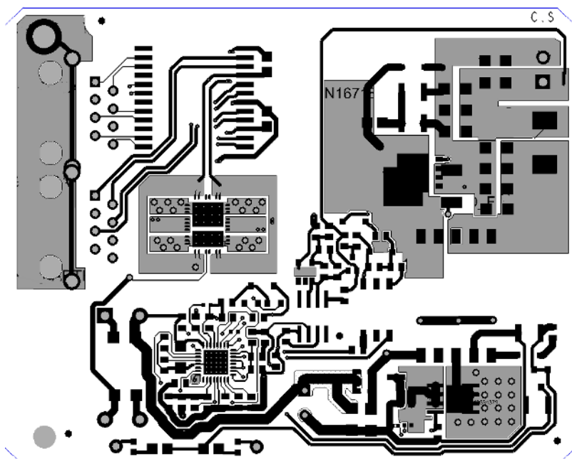
Figure 20: Top Layer
