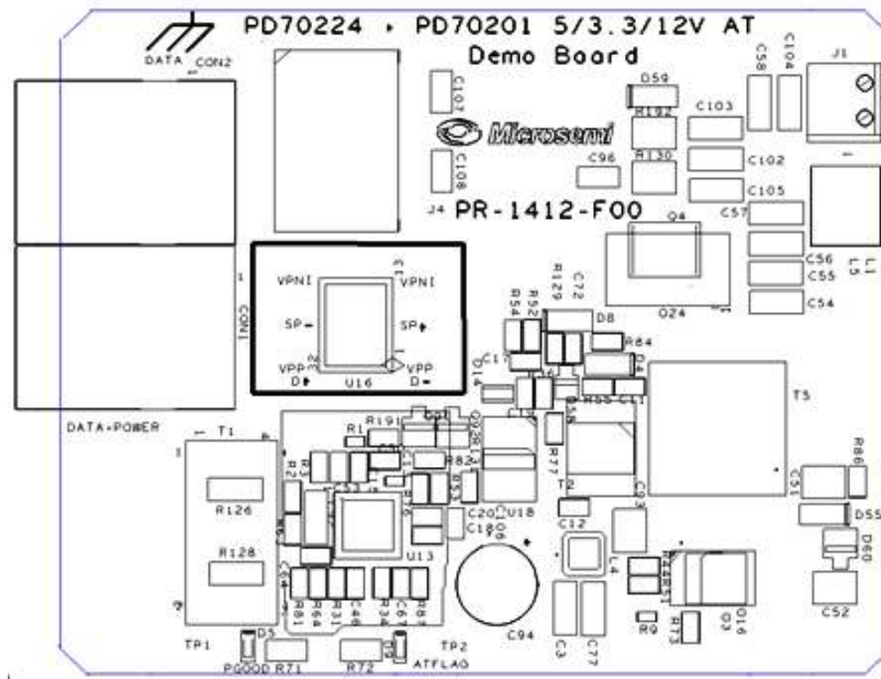
Figure 19: Top Silk
