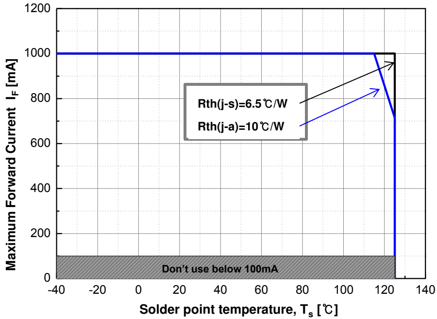
Fig 9. Maximum Forward Current vs. Solder point temperature, T_j (max.)=150°C
