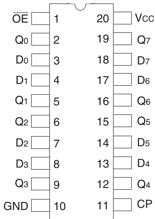
CERDIP/ SSOP/ QSOP TOP VIEW
