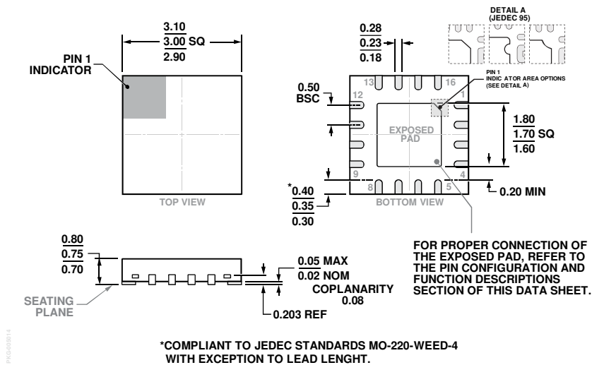
Figure 60. 16-Lead Lead Frame Chip Scale Package [LFCSP] 3 mm x 3 mm Body and 0.75 mm Package Height (CP-16-48)
