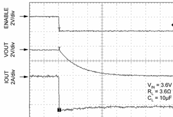
Turn-Off Timing
