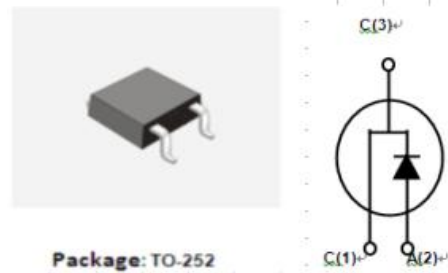
Package: TO-252
