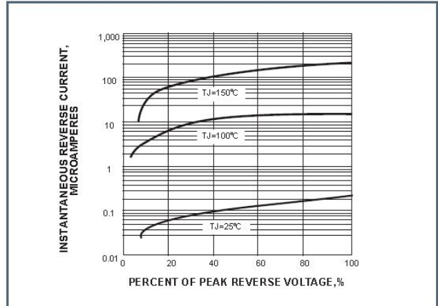
FIG. 4-TYPICAL REVERSE CHARACTERISTICS
