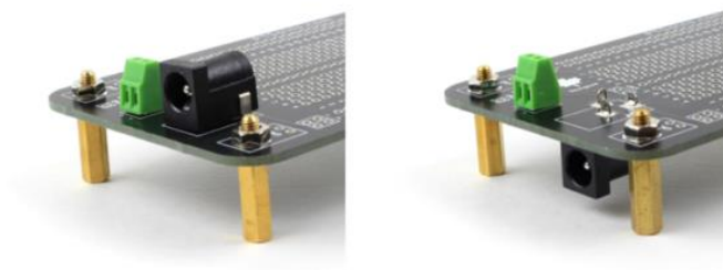
Figure 13: Power input configuration examples.
