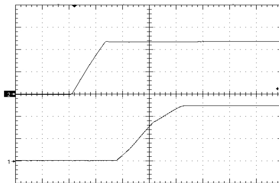
Figure 10. Startup Waveform via Line Voltage, time scale 4mS/div. Vin=Vin_nom, Iout=full load Cout=0uF, Ch1=Vout (2V/div), Ch2=Vin (20V/div)
