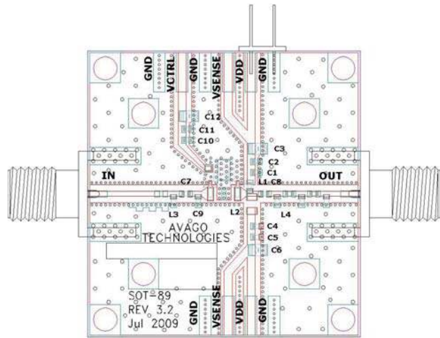
Figure 26. Demoboard
