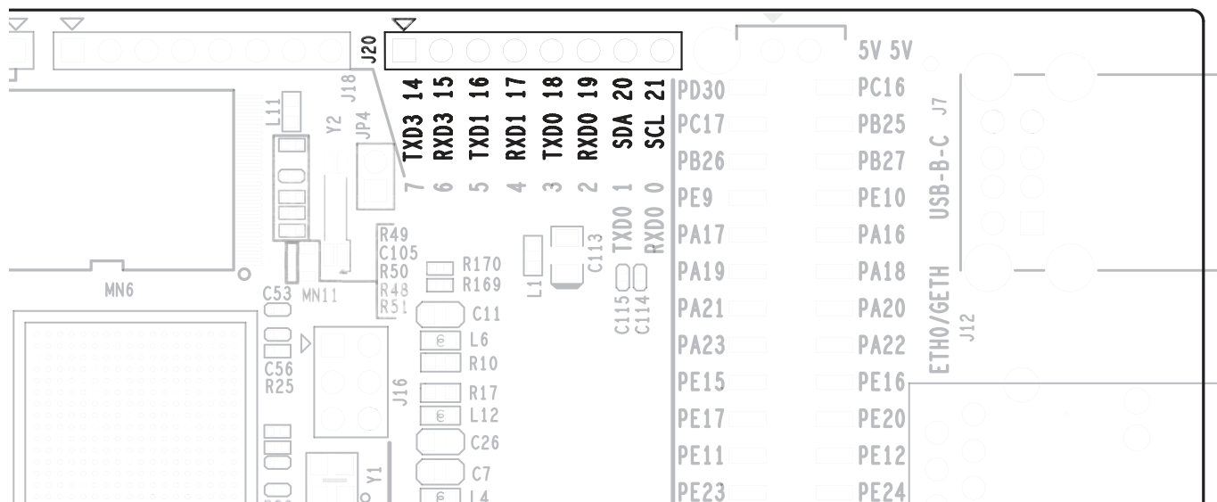
Figure 4-22. J20 Header
