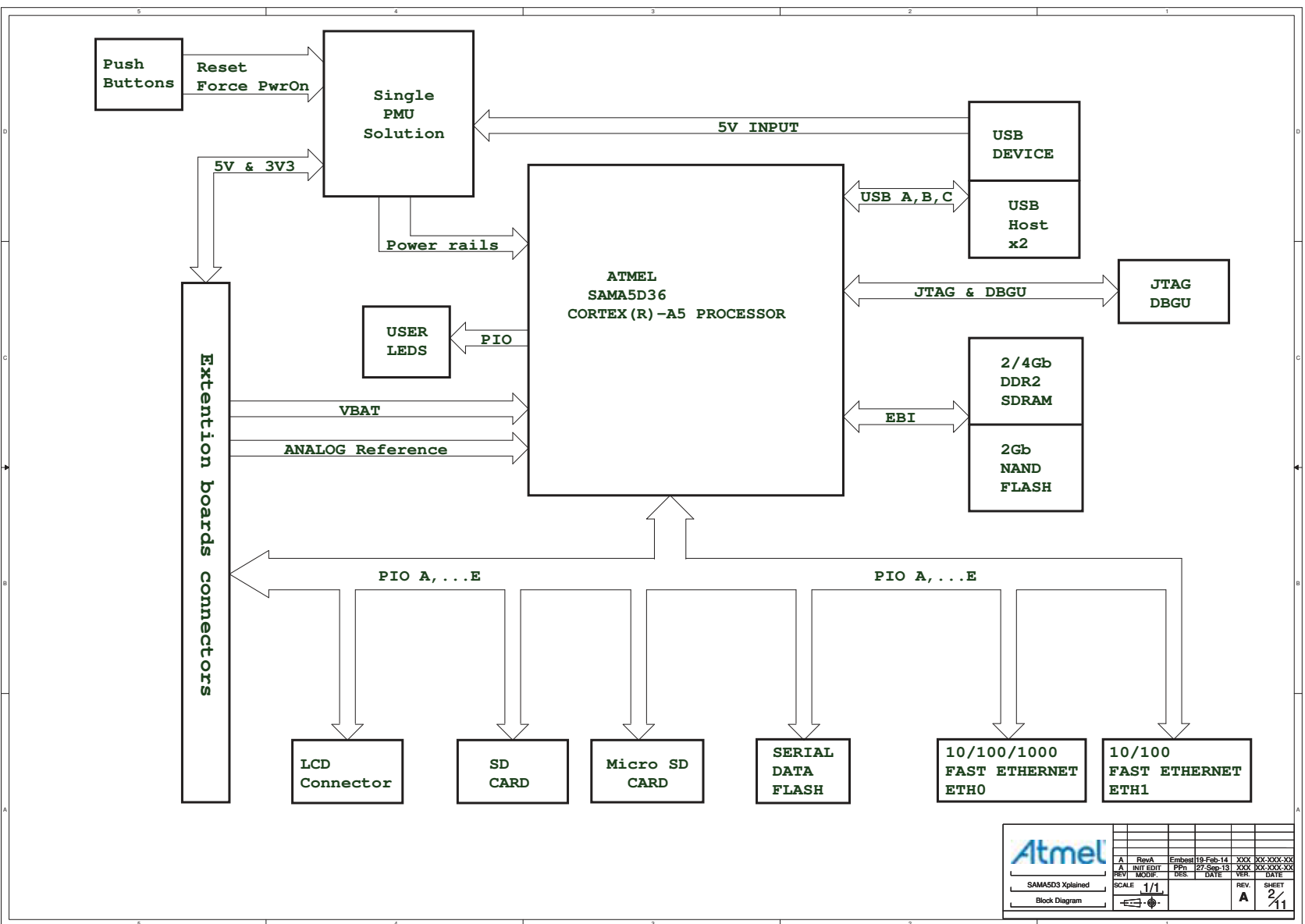
Figure 4-39. Block diagram
