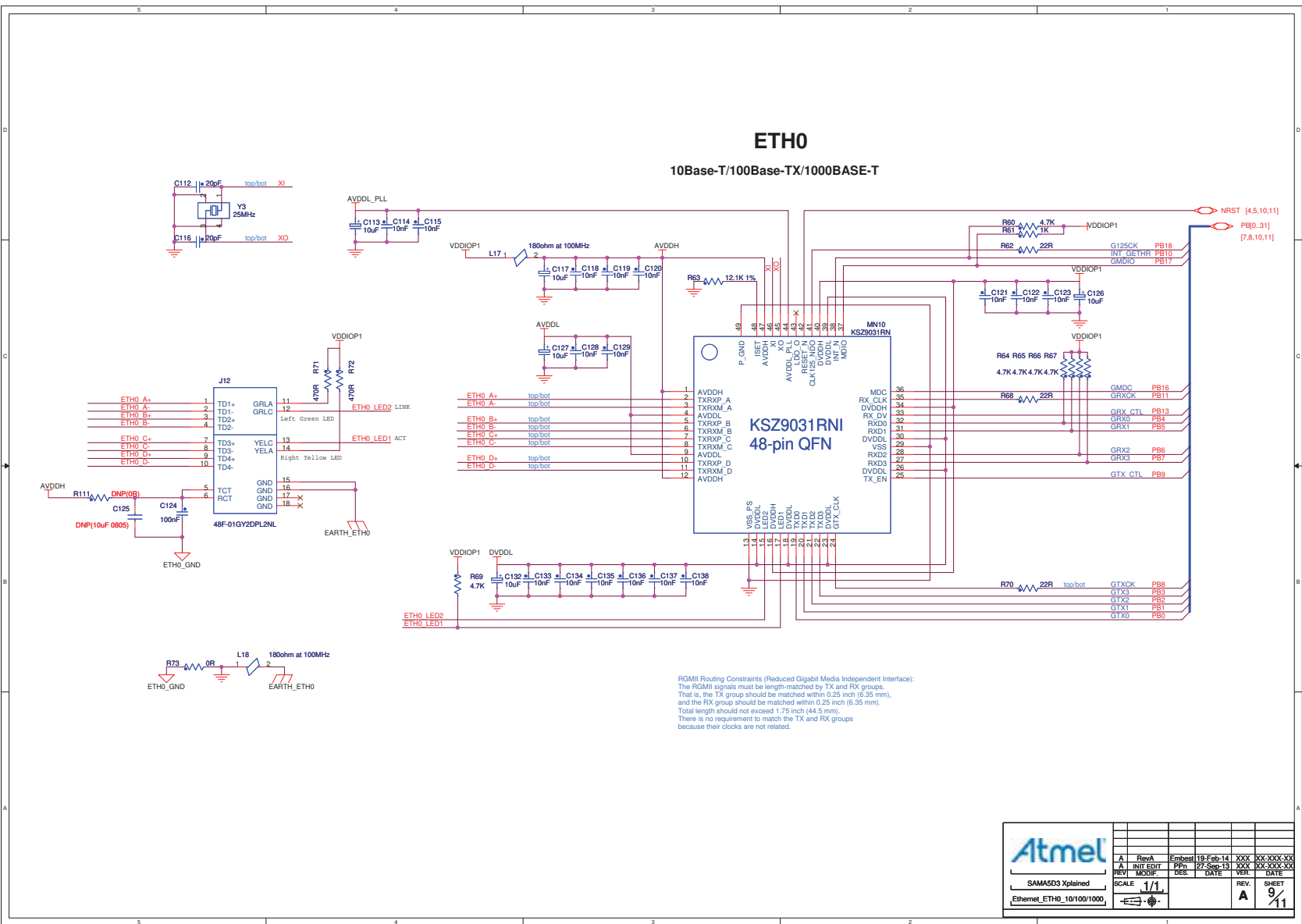
Figure 4-46. Gigabit Ethernet
