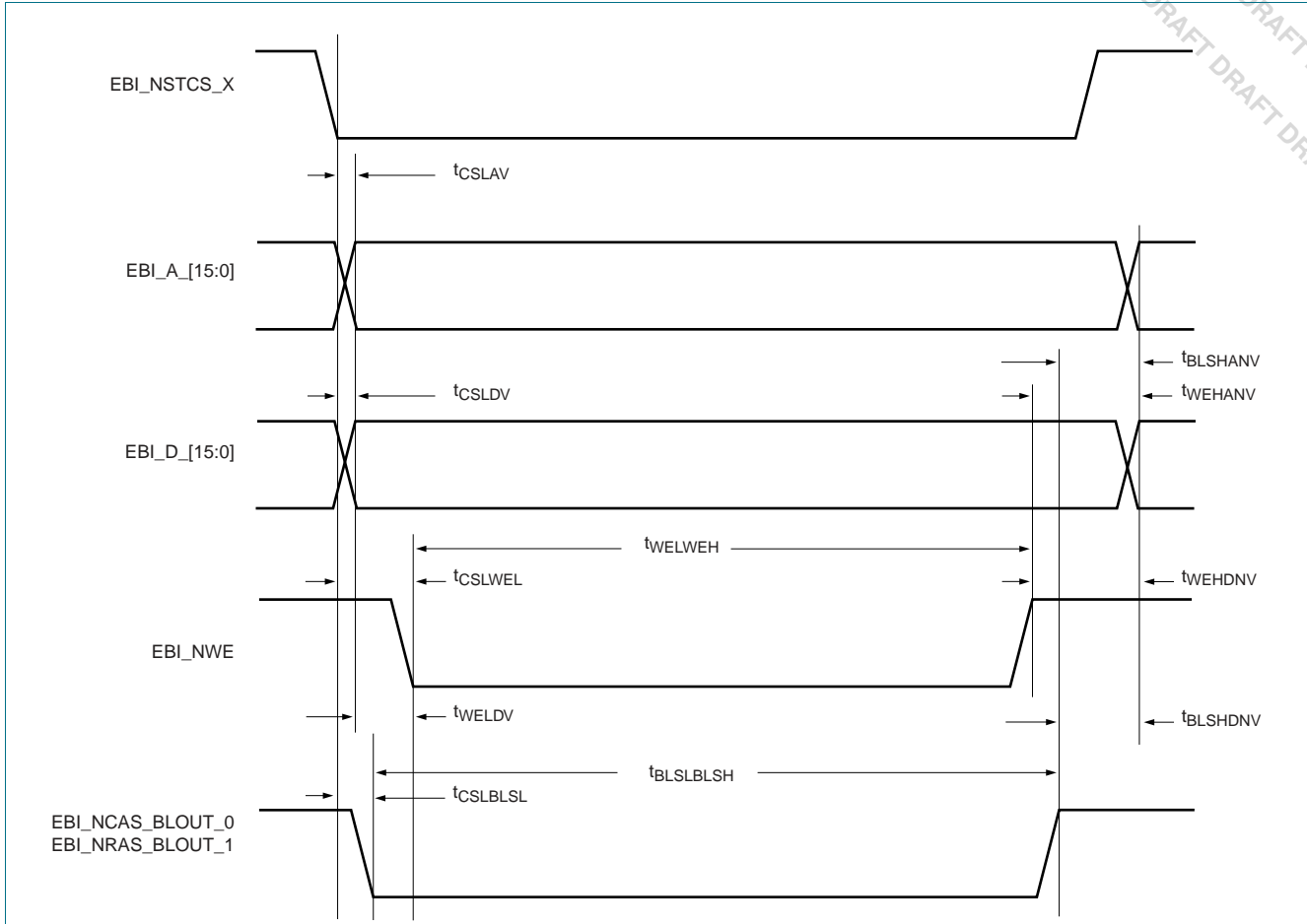
Fig 22. External memory write access to static memory
