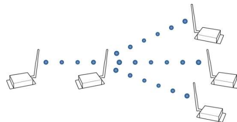
Figure 5.5. Sample Repeater Network Topology
