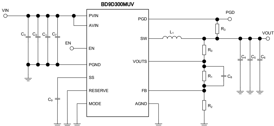
Figure 60. Application Circuit
