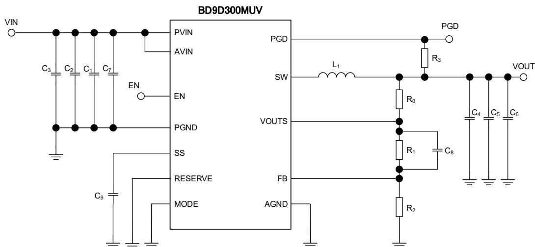
Figure 35. Application Circuit
