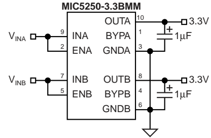
Figure 2. Low-Noise Fixed Voltage Application
