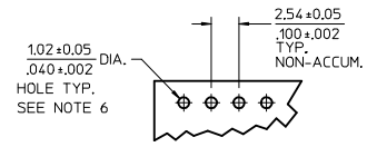
TYP. HOLE PATTERN FOR 1.57/.062 THK. PCB
